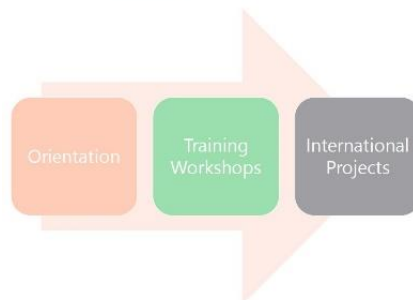
Program Components
