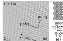
TEM microscope image of nano structures prepared at our Lab.
