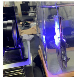
Photocatalytic activity of \text{TiO}_2 -based materials can generate electricity by oxidatively degrading one of organic wastes, cellulose, during light irradiation.
