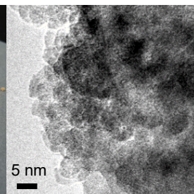
Transmission electron microscope (TEM) image of allophane nanoparticles.
