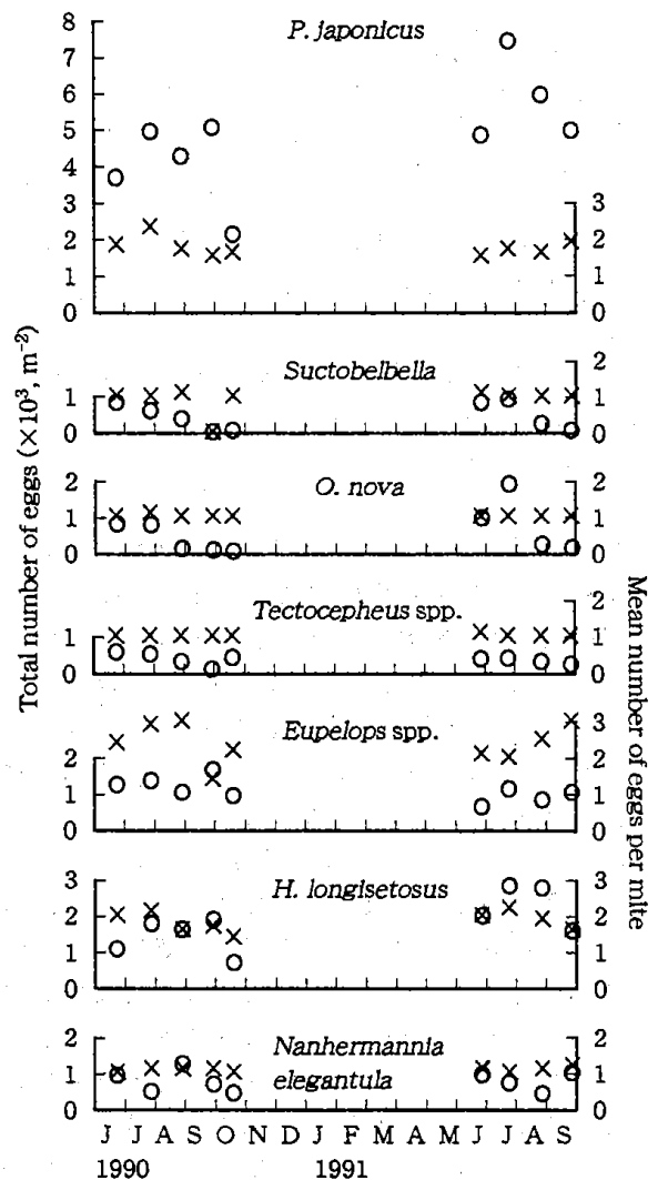
Fig. 6. Seasonal change in mean number of eggs in a gravid females (x) and total number of eggs per m² (o) for each of major oribatid species.
