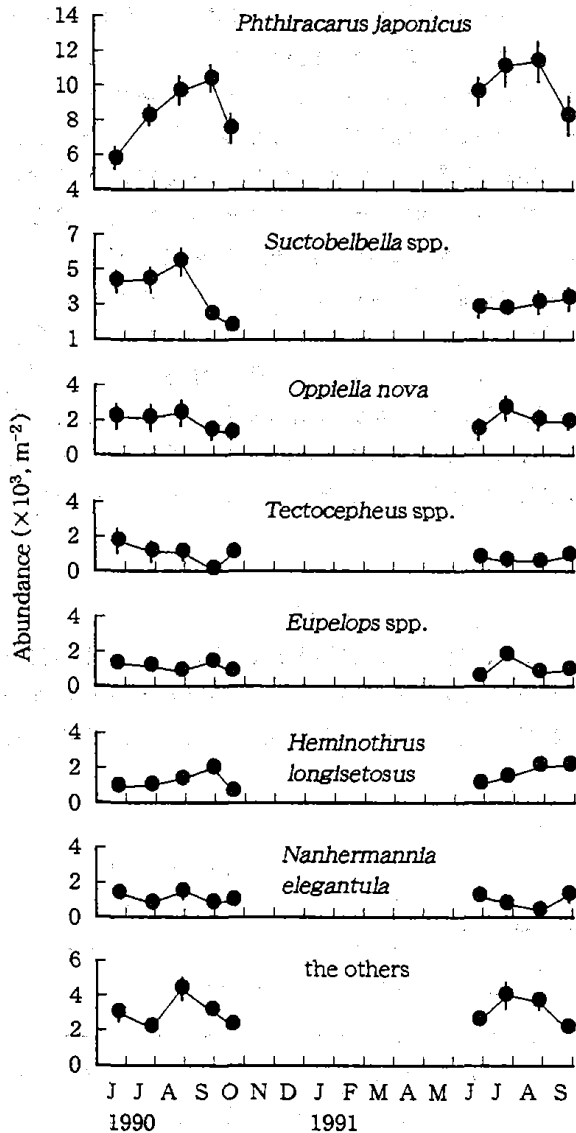
Fig. 2. Seasonal change in abundance of major oribatid mites.
